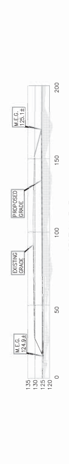
SECTION D-D SCALE IS 1" = 20'
