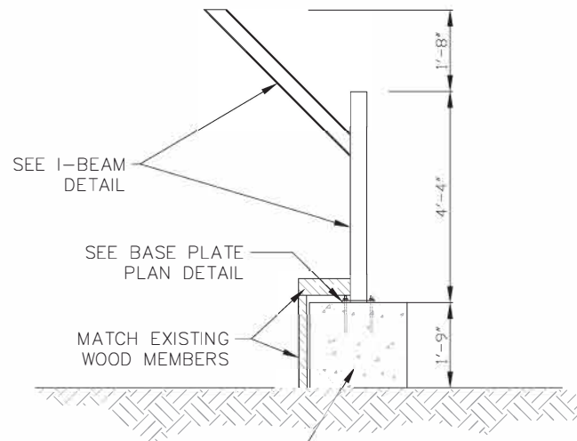
24" SQUARE X 21" DEPTH CONCRETE FOUNDATIONS SPACED ON 97" CENTERS
